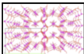
Fig. 2. A schematic representation of a section of the three-dimensional network in a projection along [001]. Hydrogen atoms are omitted for clarity.
